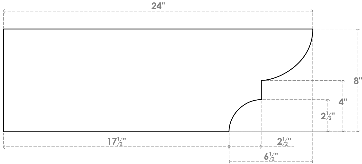
SIDE PROFILE
